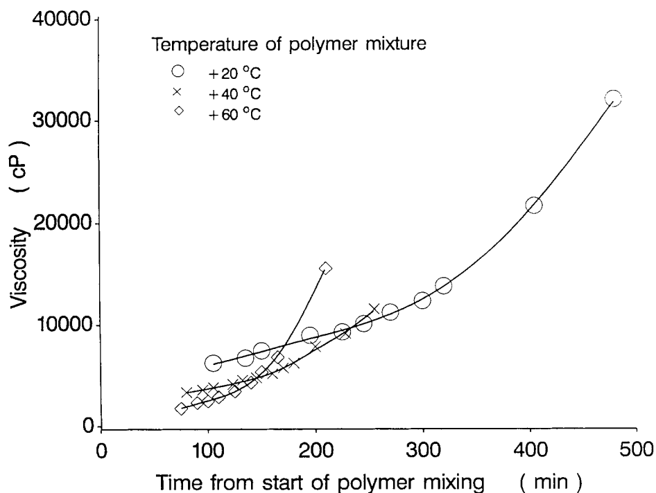
Figure 6 Viscosity development of polymer mix at different temperatures.
